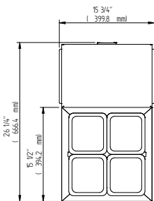
CPR-4 Top View
