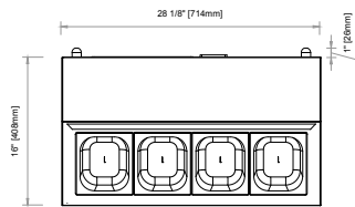
CPR-4 Top View
