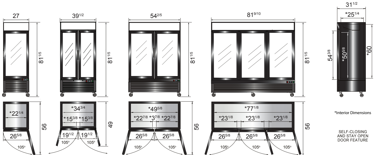
MCF8722GR
