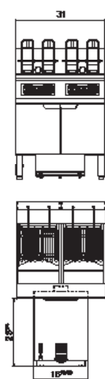
AEFF-50-2TB
