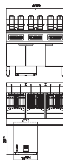
AEFF-50-3B
