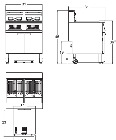
AEFF-50-2T
