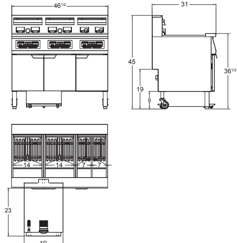
AEFF-50-3T
