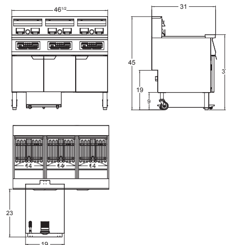
AEFF-50-3T
