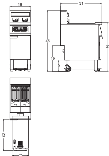
AEFF-50-1T
