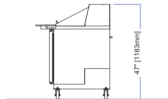
Closed Lid
