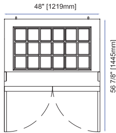
APT-48-18 Front
