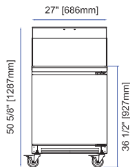
APT-27-12 Front
