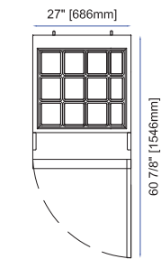
APT-27-12 Front
