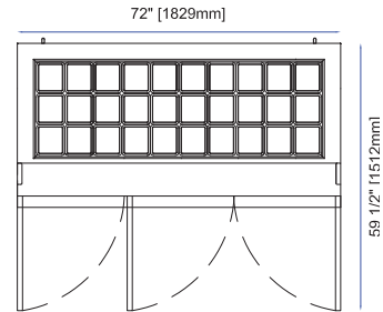
APT-70-32 Front
