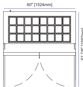
APT-60-24 Front
