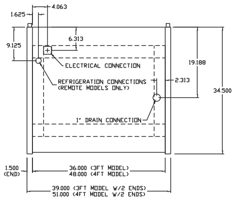
3' & 4' PLAN VIEWS
